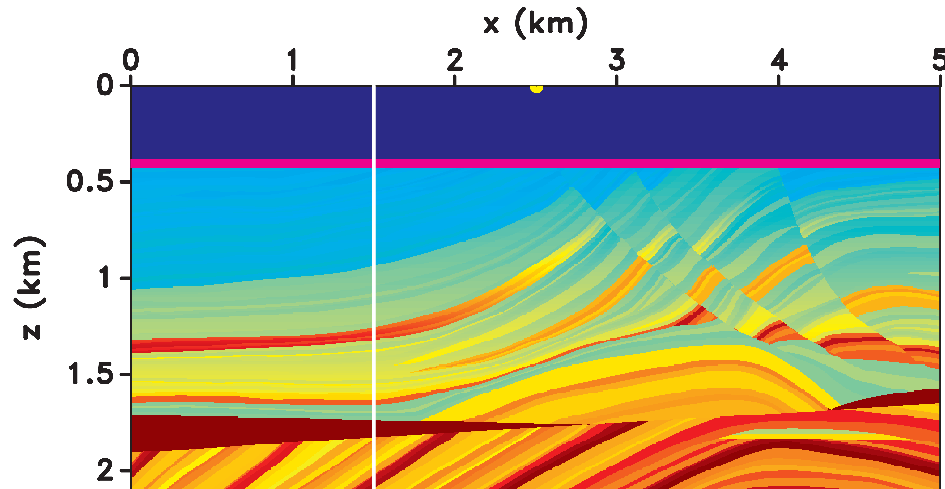
Density model
